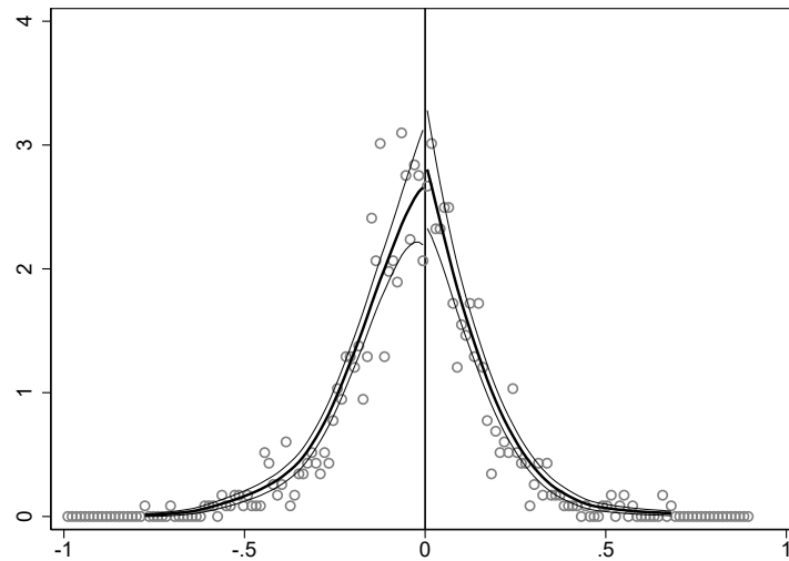
Figure A3: McCrary (2008) 's density test
