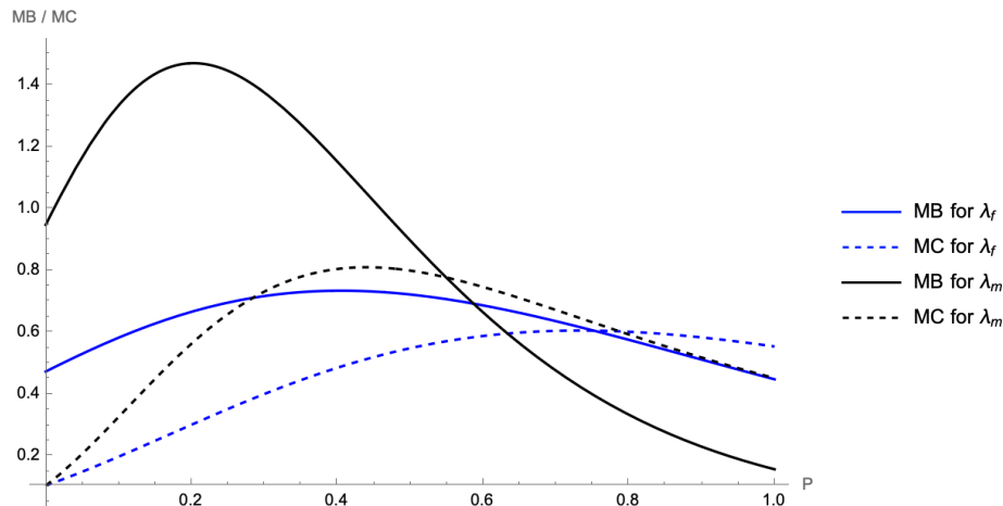
Figure E2: Marginal benefits and marginal costs of the policy at high levels of belief in the shock ( p = 0.75 )
